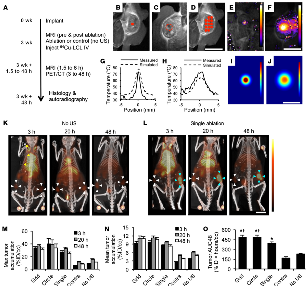
Figure 1. MRgFUS ablation enhanced accumulation of 64 Cu-LCL in NDL mammary carcinoma. (A) Three weeks after tumor implantation, tumors were ablated and imaged with pre- and postablation T1w-MRI. Mice were then injected with i.v. 64 Cu-LCL and imaged with PET-CT at 3, 20, and 48 hours after treatment. Control treatment was no ultrasound (no US). (B–J) MRgFUS protocols and temperature profiles. T1w images localize ultrasound for (B) single-point, (C) circle, and (D) grid protocols. MR thermometry images following (E) 20 seconds single-point or (F) 60 seconds circle protocol MRgFUS. Temperature of measured and simulated ultrasound focus is plotted after (G) 20 seconds single-point or (H) 60 seconds circle protocol. Temperature distribution was simulated following (I) 20 seconds single-point or (J) 60 seconds circle protocol. Grid protocol shown in D and M–O is equivalent to E and G repeated in grid pattern, due to sequential application of ablation points and cool-down period. (K) PET-CT maximum intensity projection images of 64 Cu-LCL without ablation. White arrows indicate tumors; yellow arrowheads indicate jugular vein (JV), heart (H), and liver (L). (L) At 3, 20, and 48 hours following single-point ablation (blue arrows), liposome accumulation is enhanced as compared with that in contralateral tumors (white arrows) in PET-CT images. 64 Cu-LCL PET image-derived volume of interest analysis plotted as (M) maximum voxel intensity, (N) average activity, and (O) AUC 48 . Significance is analyzed with 1-way ANOVA followed by Tukey’s test. For M–O, n = 4, 3, 12, 19, and 6 mice for grid, circle, single point, contralateral tumors (contra), and no treatment. Scale bars: 1 cm. Thermometry color bars range from 70°C to 40°C; PET color bar ranges from 25%ID/cc to 0%ID/cc. *P < 1 × 10 −4 vs. untreated tumors; †P < 0.05 vs. single-point ablation. Data are pooled from 5 experiments.
